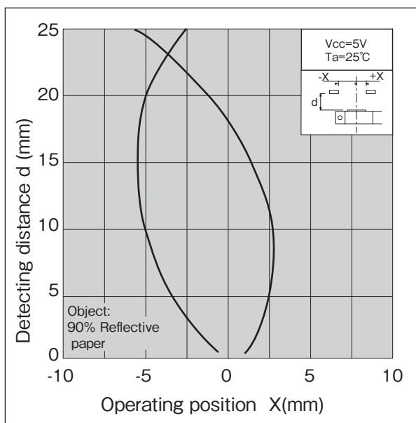
Operating Position vs Detecting Distance (typ. - 2-)
