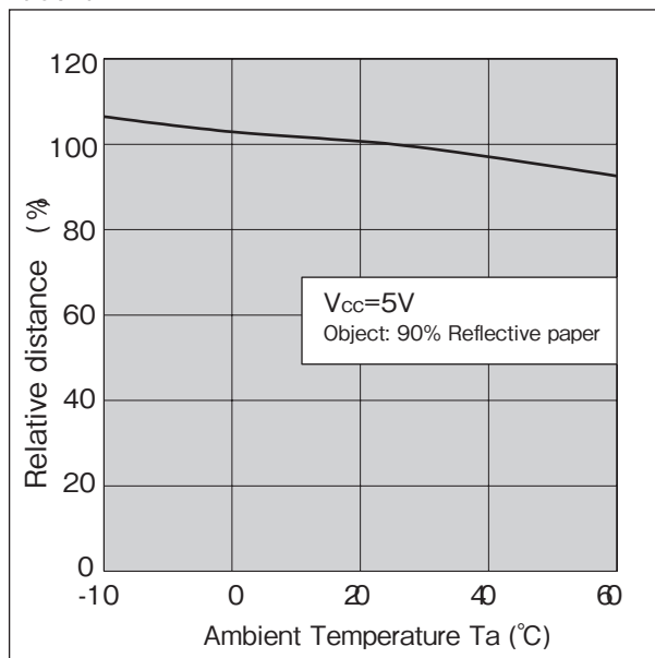
Detecting Distance vs Ambient Temperature (typ.)
