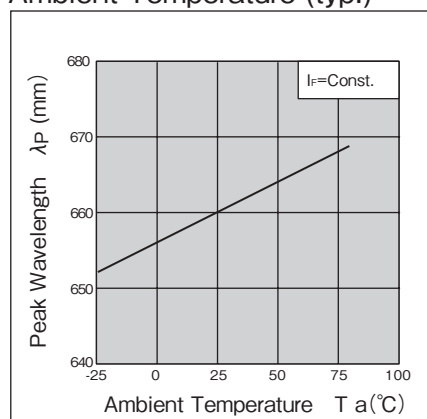
Peak Wavelength vs. Ambient Temperature (typ.)
