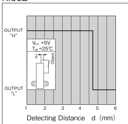
Detecting Position 1 (typ.) KI662
