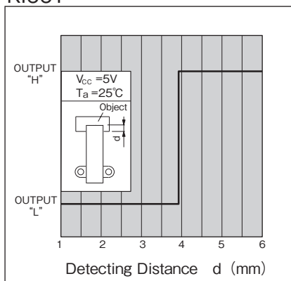
Detecting Position 2 (typ.) KI661
