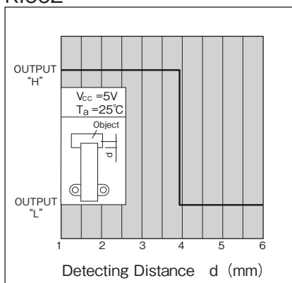
Detecting Position 2 (typ.) KI662
