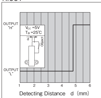
Detecting Position 1 (typ.) KI661
