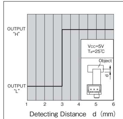
Detecting Position 2 (typ.) KI1258
