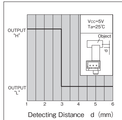
Detecting Position 2 (typ.) KI1257
