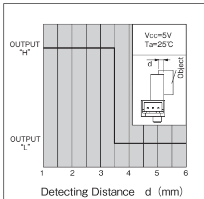
Detecting Position 1 (typ.) KI1257
