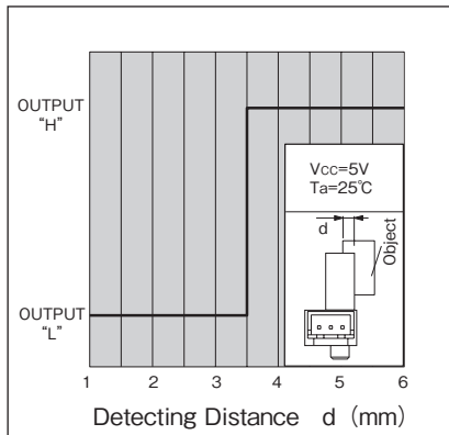
Detecting Position 1 (typ.) KI1258
