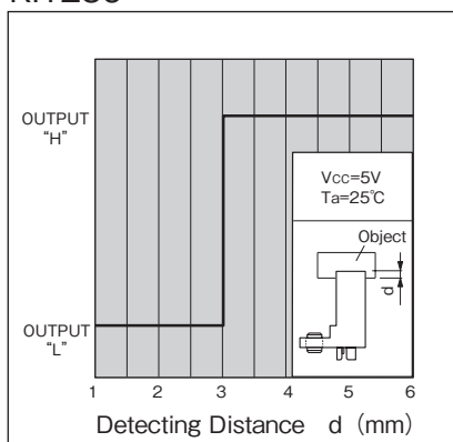
Detecting Position 2 (typ.) KI1236
