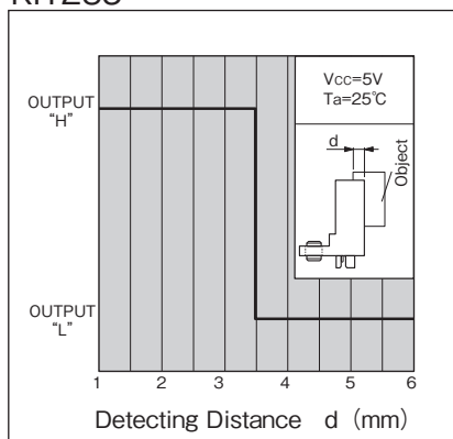
Detecting Position 1 (typ.) KI1235
