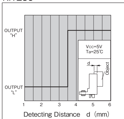
Detecting Position 1 (typ.) KI1236
