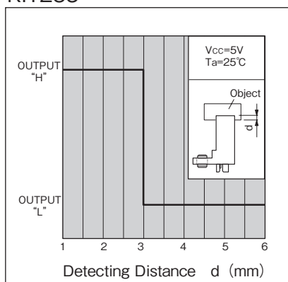
Detecting Position 2 (typ.) KI1235
