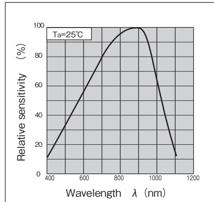
Spectral Sensitivity (typ.)
