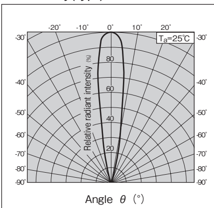
Directivity (typ.)
